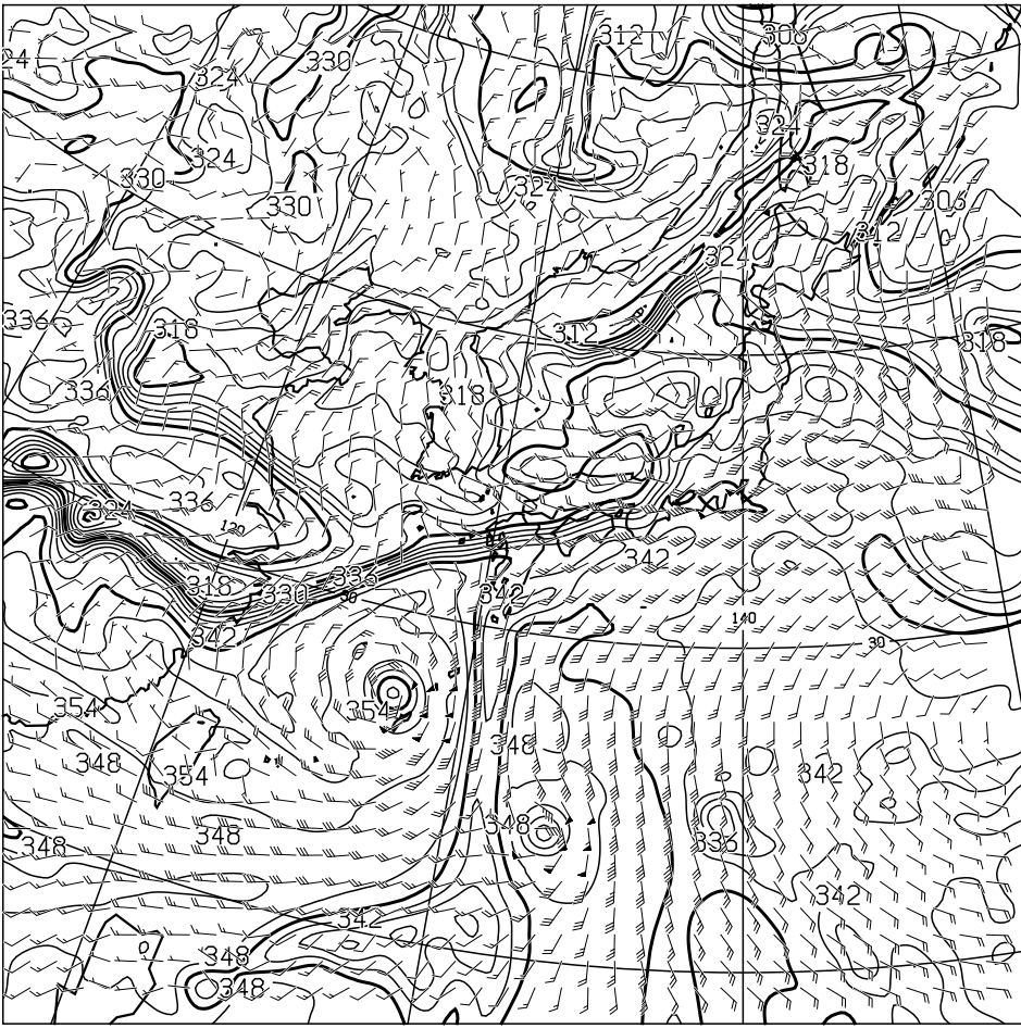
T=12 850hPa: E.P. TEMP (K), WIND (KNOTS) VALID 260000UTC
