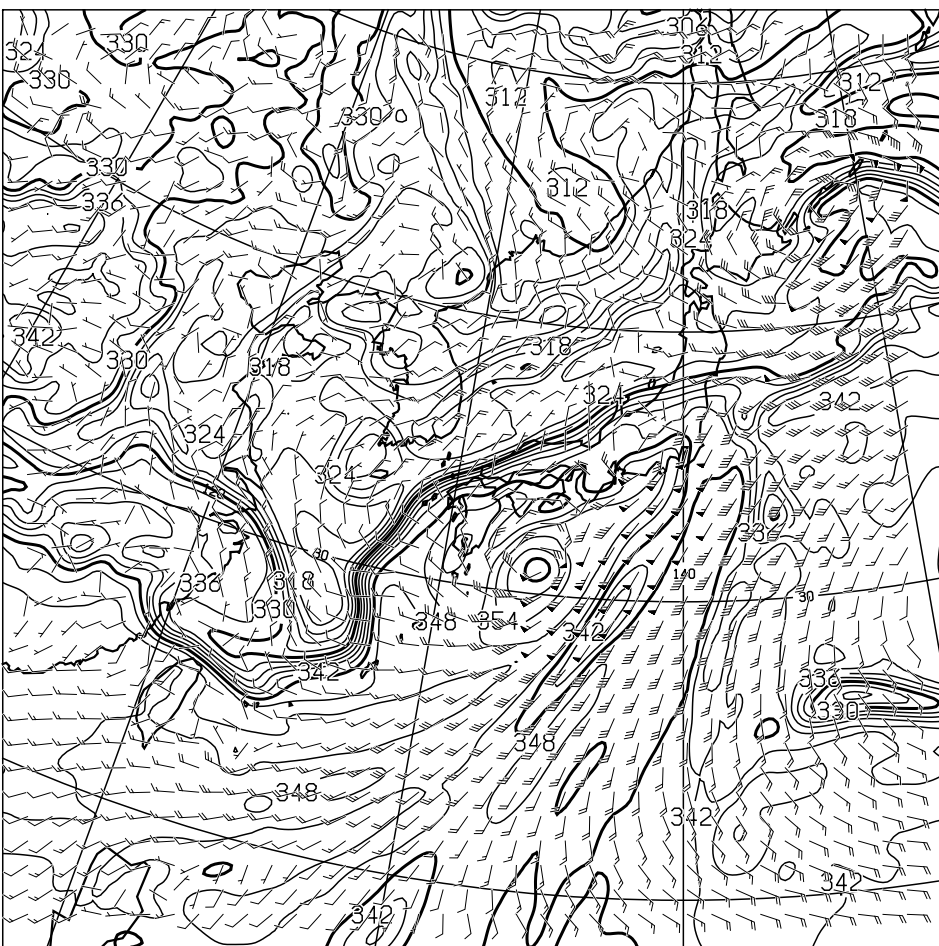
T=36 850hPa: E.P. TEMP (K), WIND (KNOTS) VALID 270000UTC
