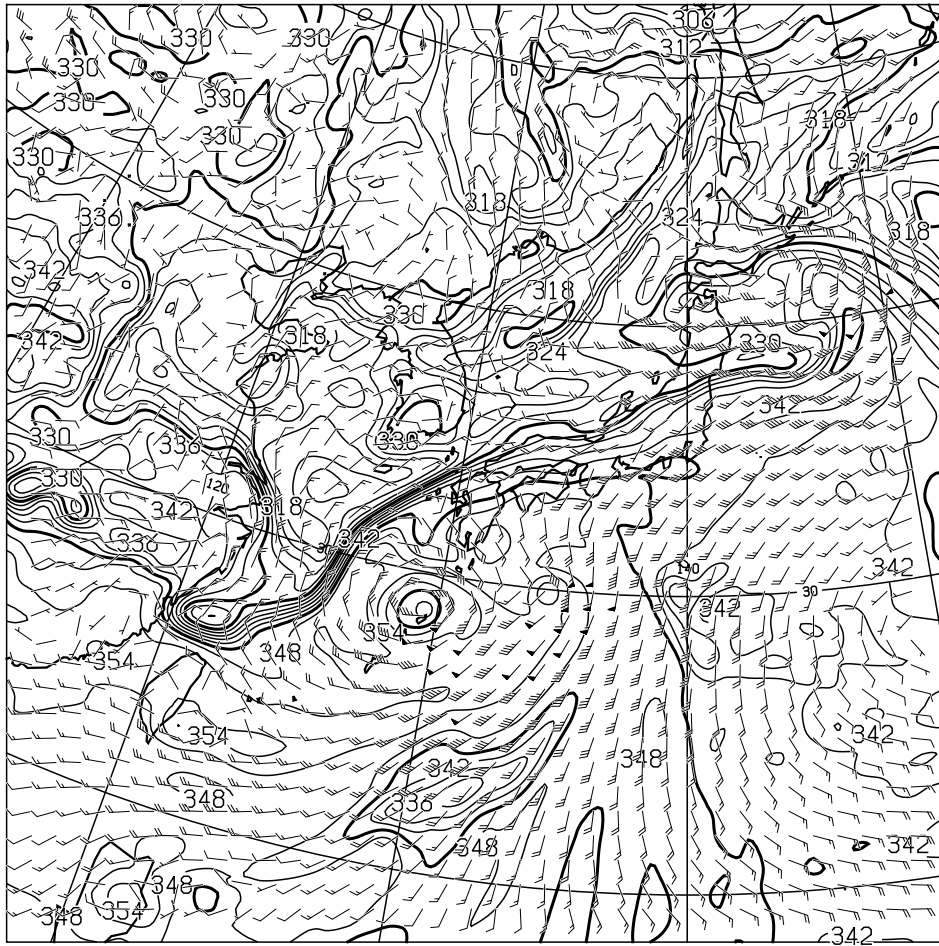
T=24 850hPa: E.P. TEMP (K), WIND (KNOTS) VALID 261200UTC
