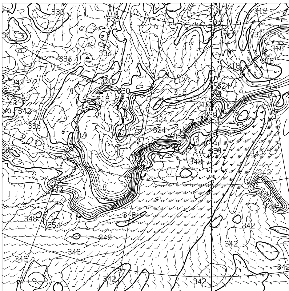
T=48 850hPa: E.P. TEMP (K), WIND (KNOTS) VALID 271200UTC
