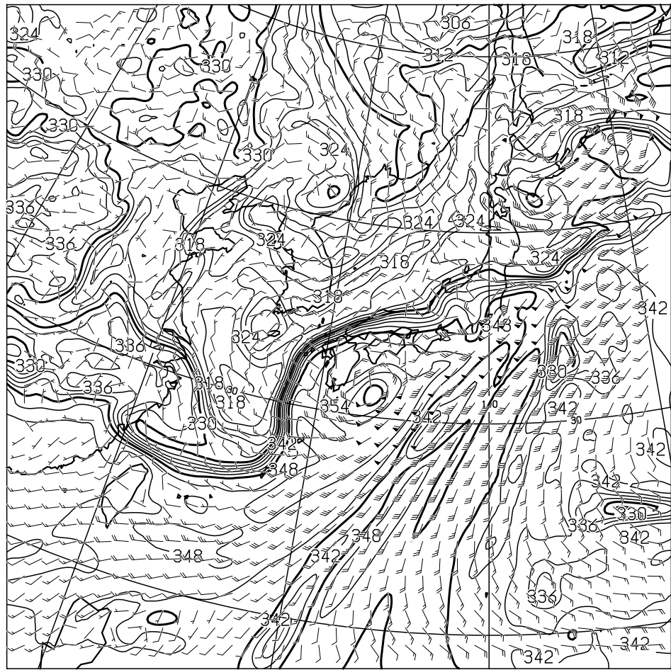
T=24 850hPa: E.P. TEMP(K), WIND(KNOTS) VALID 270000UTC
