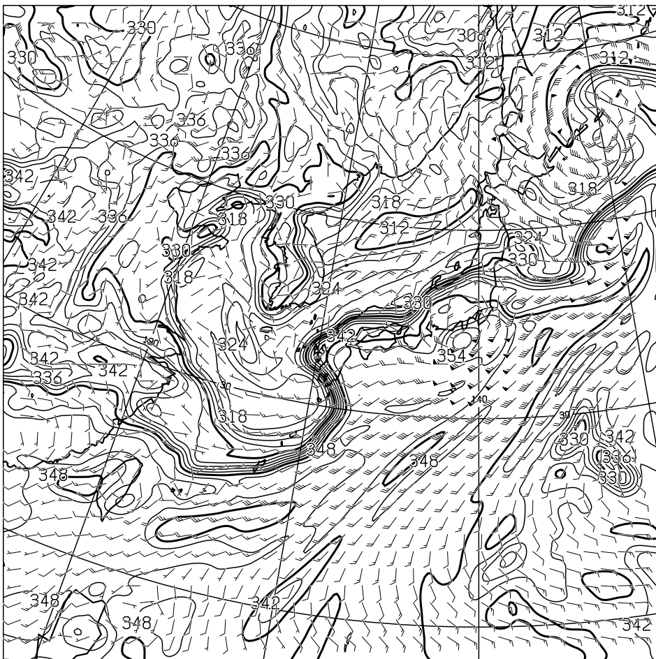
T=36 850hPa: E.P. TEMP(K), WIND(KNOTS) VALID 271200UTC
