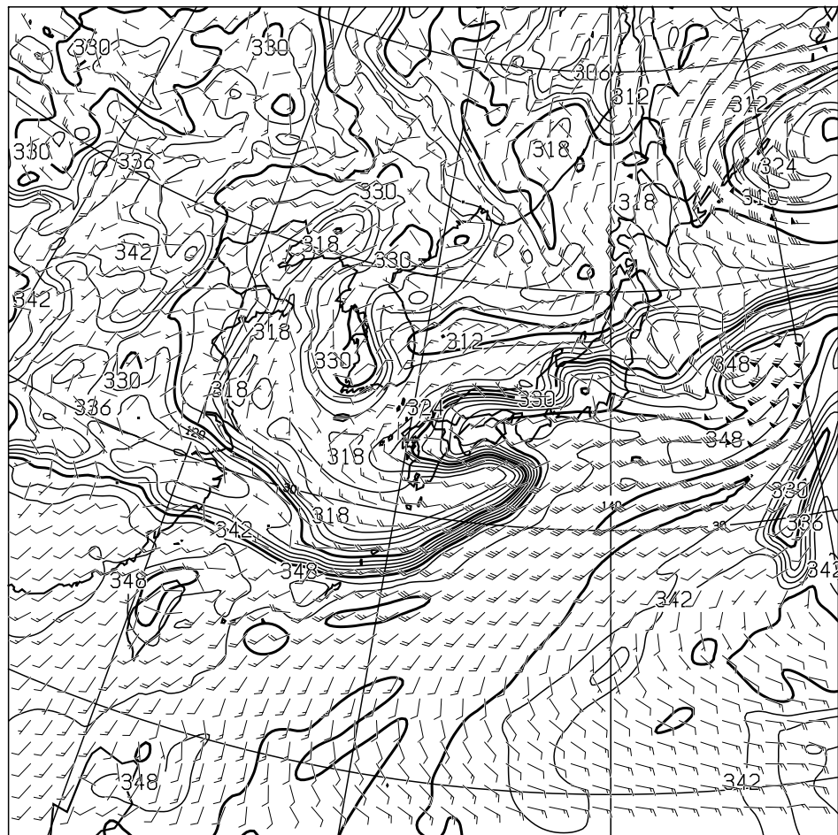
T=48 850hPa: E.P. TEMP(K), WIND(KNOTS) VALID 280000UTC
