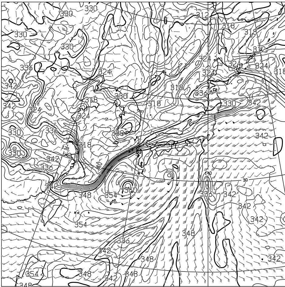
T=12 850hPa: E.P. TEMP(K), WIND(KNOTS) VALID 261200UTC
