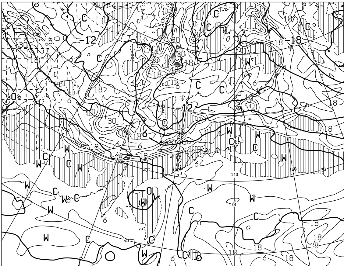
T=12 VALID 251200UTC TEMP (C) AT 500hPa T-TD (C) AT 700hPa
