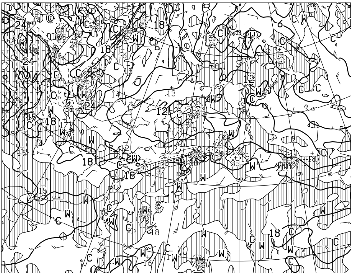
T=12 VALID 251200UTC TEMP (C), WIND ARROW AT 850hPa P-VEL (hPa/H) AT 700hPa
