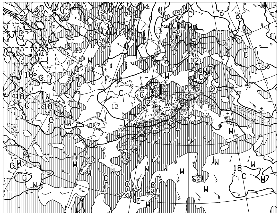
T=24 VALID 260000UTC TEMP (C), WIND ARROW AT 850hPa P-VEL (hPa/H) AT 700hPa
