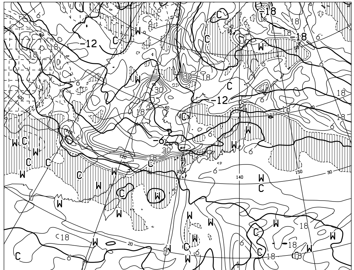
T=24 VALID 260000UTC TEMP (C) AT 500hPa T-TD (C) AT 700hPa
