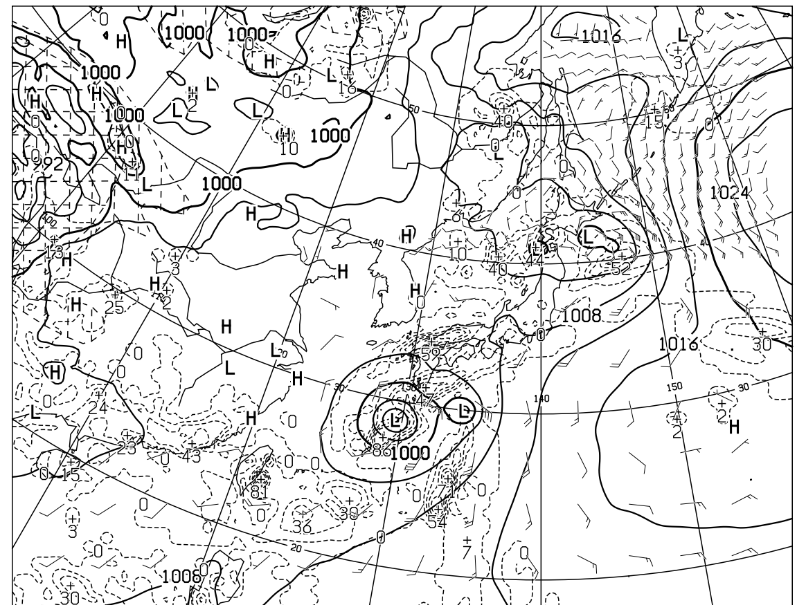
T=24 VALID 261200UTC SURFACE PRESS (hPa), PRECIP (MM) (12-24) WIND ARROW AT SURFACE
