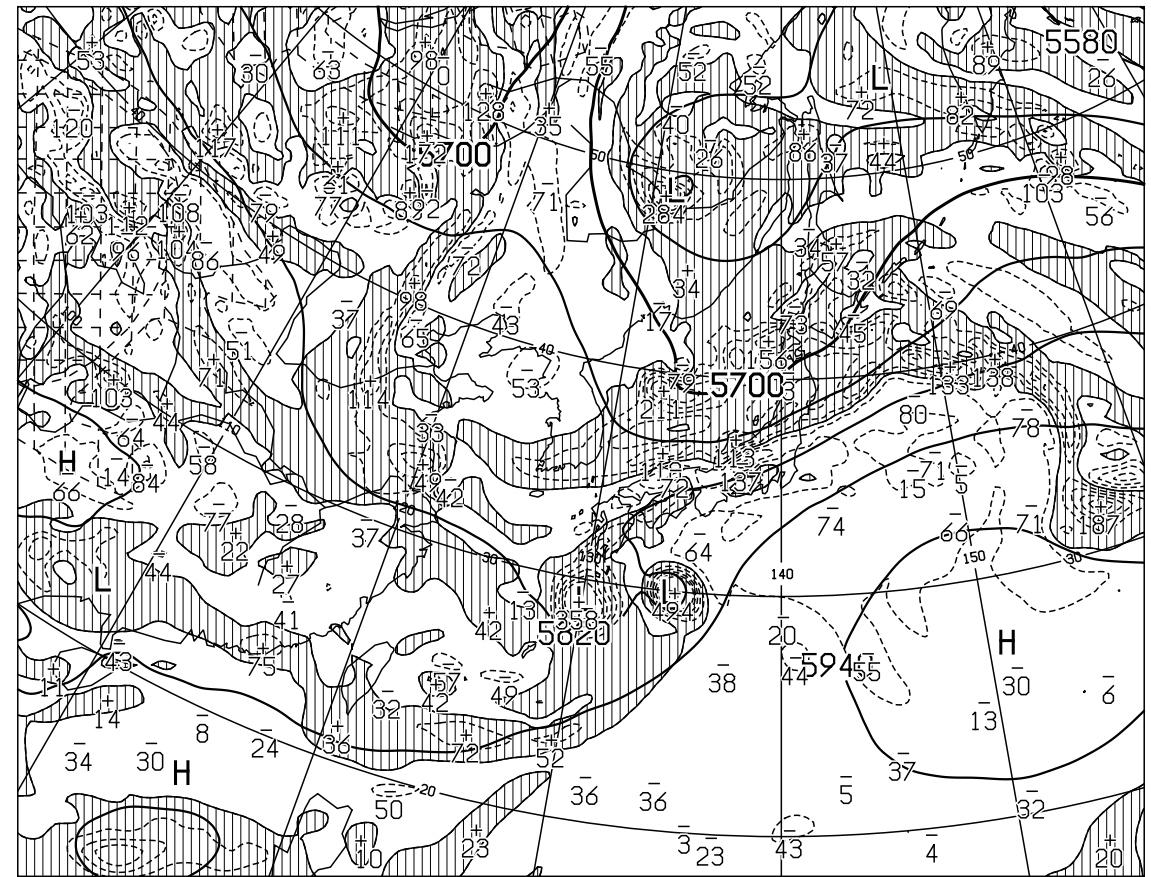
T=24 VALID 261200UTC HEIGHT (M), VORT (10 x -6/SEC) AT 500hPa
