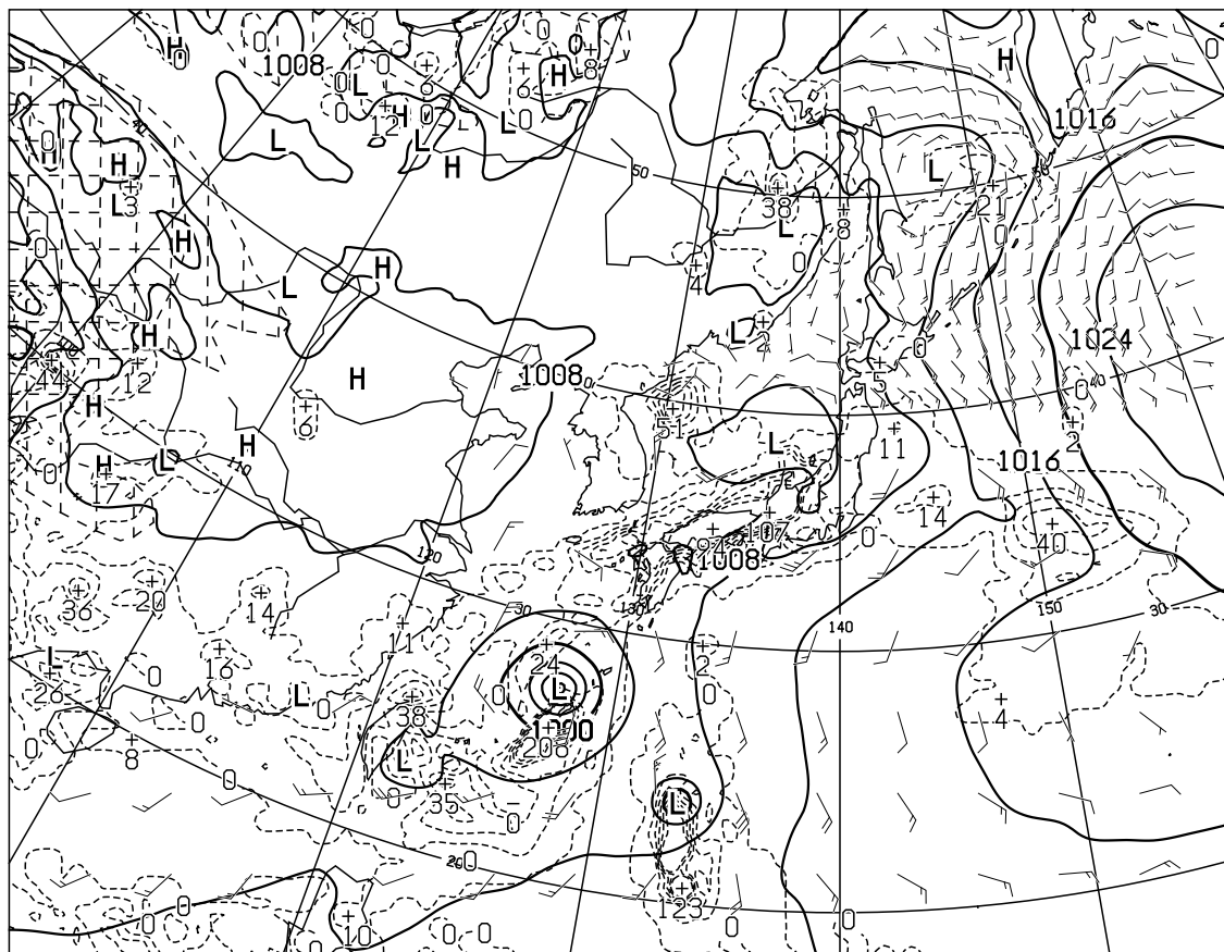
T=12 VALID 260000UTC SURFACE PRESS (hPa), PRECIP (MM) (00-12) WIND ARROW AT SURFACE
