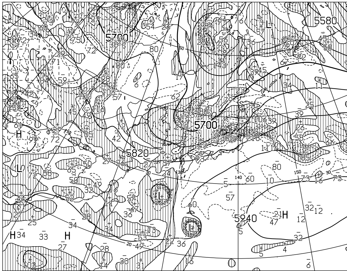
T=12 VALID 260000UTC HEIGHT (M), VORT (10 x -6/SEC) AT 500hPa
